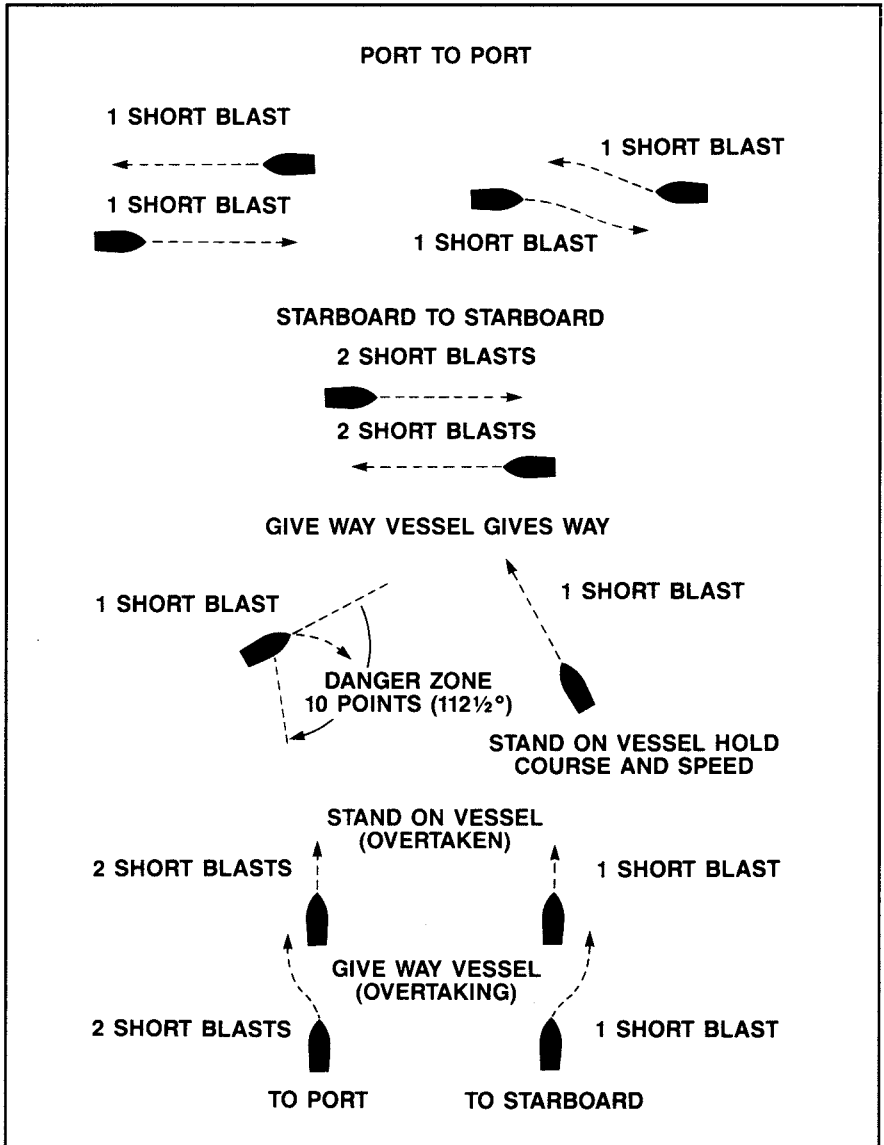
Standard sound signals
