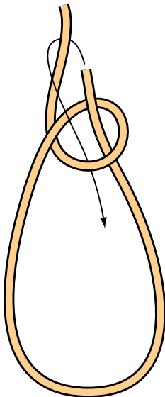
Bowline
