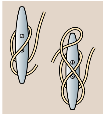
Making fast to a cleat
