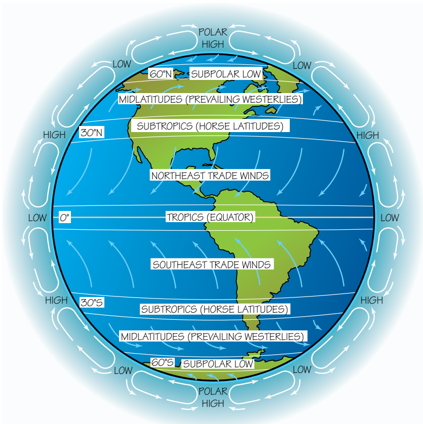
This global winds diagram shows wind’s basic patterns. The actual patterns of wind at any given moment are far more complicated.
