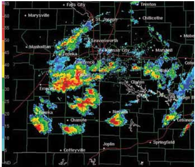
Dark areas on this radar image indicate dry air and colored areas indicate the presence of water vapor. The intensity of precipitation is indicated by spectrum color, with blue meaning light precipitation and red being the heaviest.
