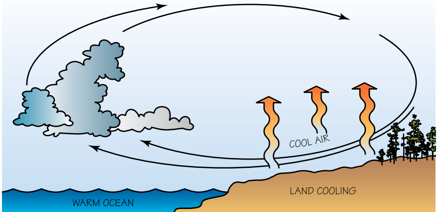
Land breezes
